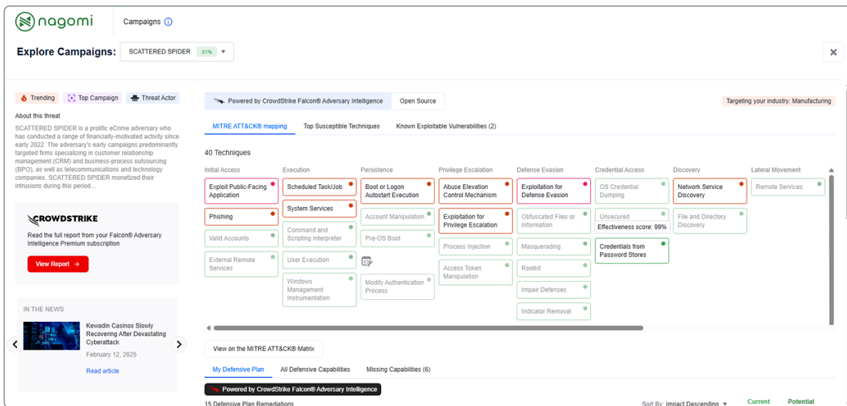
CrowdStrike-enriched MITRE Mapping
